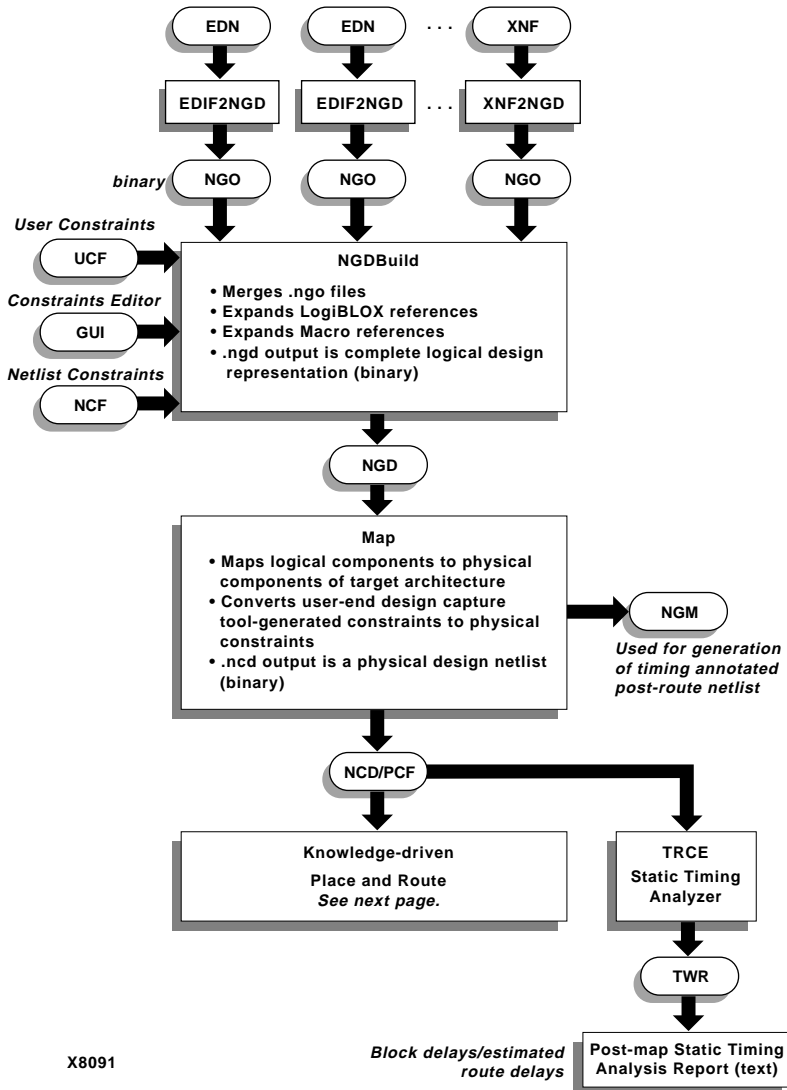
Figure D-2 Manipulation of Netlist and Constraint Files for FPGAs (Part 2)
